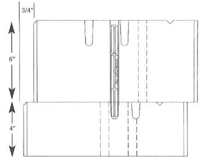
Pinning Standard/Cobble to Accent
