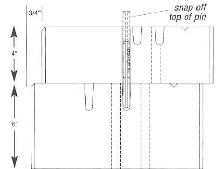
Pinning Accent to Standard/Cobble
