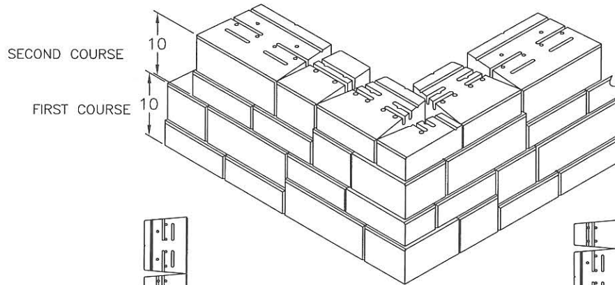
OUTSIDE 90° CORNER SCALE: NONE
