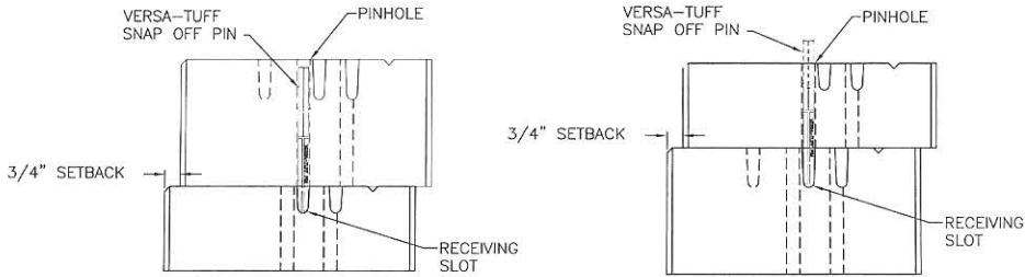
PINNING DETAIL
