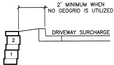
2' TALL WALL
