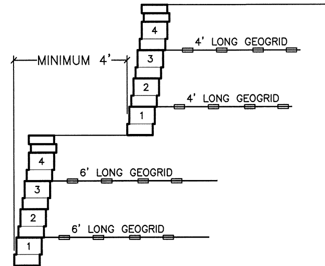
4' TIERED WALLS
