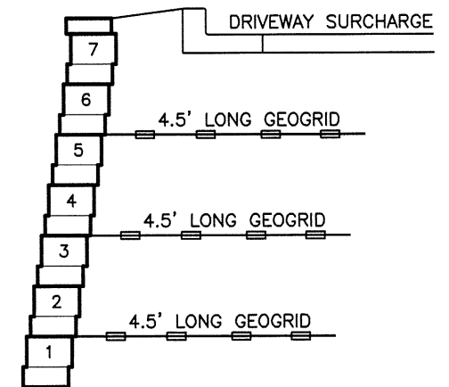
6' TALL WALL
