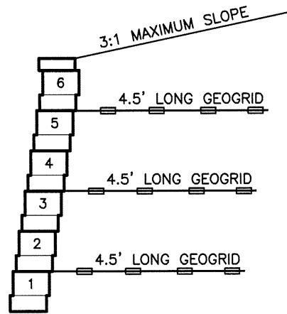
5' TALL WALL
