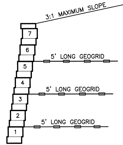
6' TALL WALL
