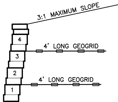
4' TALL WALL
