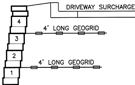
4' TALL WALL
