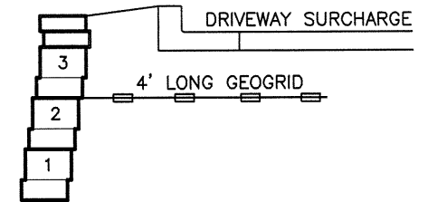
3' TALL WALL
