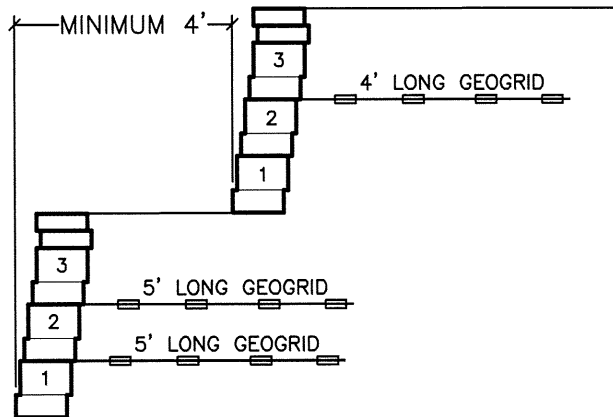
3' TIERED WALLS
