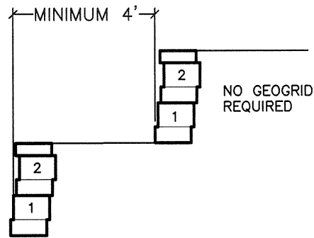
2' TIERED WALLS
