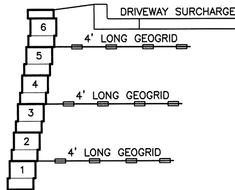
5' TALL WALL
