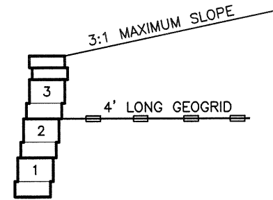
3' TALL WALL
