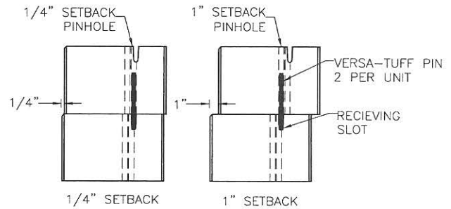
PINNING DETAIL
