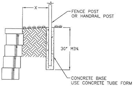
POST DETAIL TYPICAL HANDRAIL AND/OR FENCE POST SCALE: NONE
