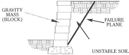
Unreinforced Wall (Figure 1A)
