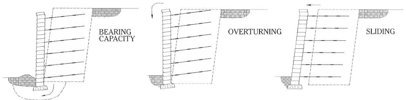
External Stability (Figure 3)
