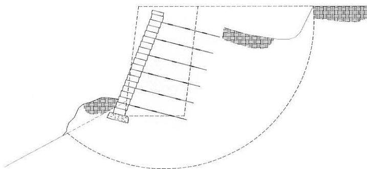
Global Stability (Figure 4)
