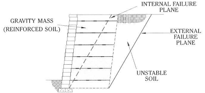
Reinforced Wall (Figure 1B)
