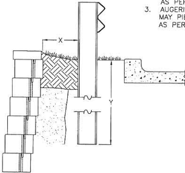
GUARD RAIL DETAIL TYPICAL GUARD RAIL SCALE: NONE
