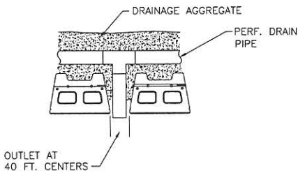
DRAIN DETAIL
