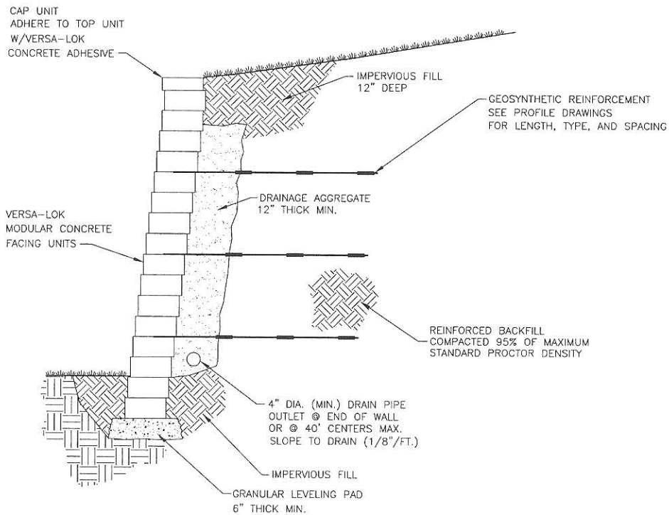
TYPICAL SECTION—REINFORCED RETAINING WALL
