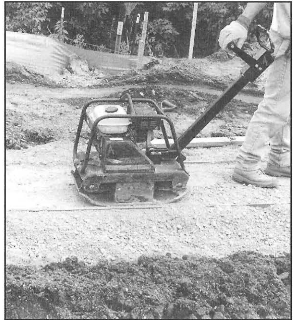
Compacted granular leveling pads provide a stiff but flexible base.
