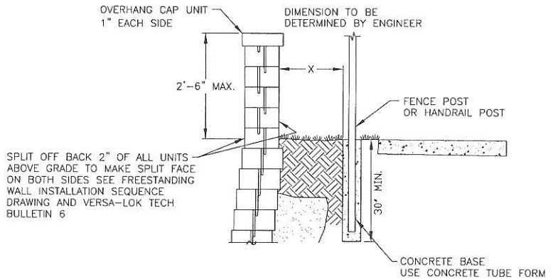
FREESTANDING WALL DETAIL (STRAIGHT WALLS ONLY) TYPICAL HANDRAIL AND/OR FENCE POST SCALE: 1/2"=1'
