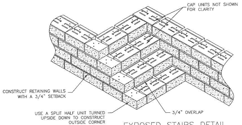
EXPOSED STAIRS DETAIL ONE SIDE EXPOSED STAIRS SCALE: NONE
