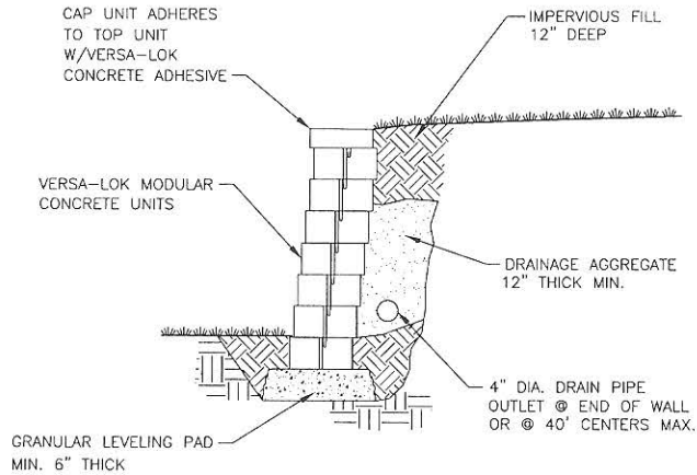
TYPICAL SECTION—UNREINFORCED RETAINING WALL
