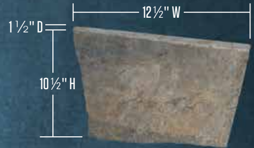
ThinCut™ Standard Quoin Dimensions
